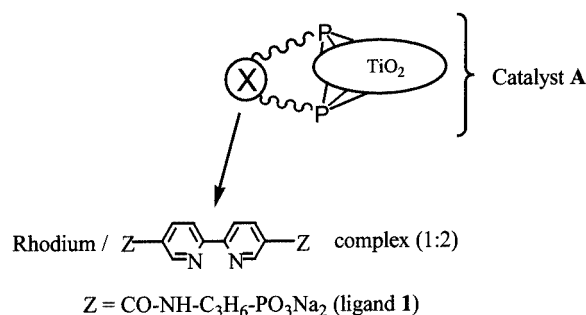
Figure 1. Schematic representation of the support bipyridine A
